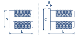
Expan/ExpanH (headed)
